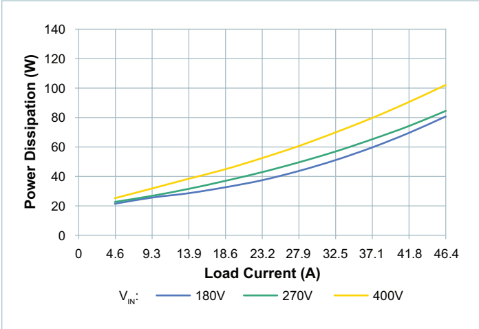
Figure 9 — Power dissipation vs. load at T_{CASE} = -40^{\circ}C , nominal trim
