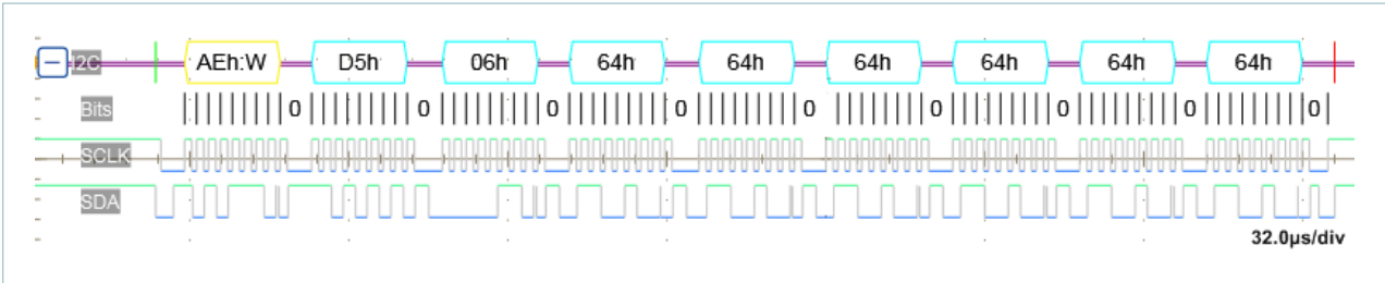
Figure 29 — SET_ALL_THRESHOLDS COMMAND (D5h)_WRITE BLOCK PROTOCOL
