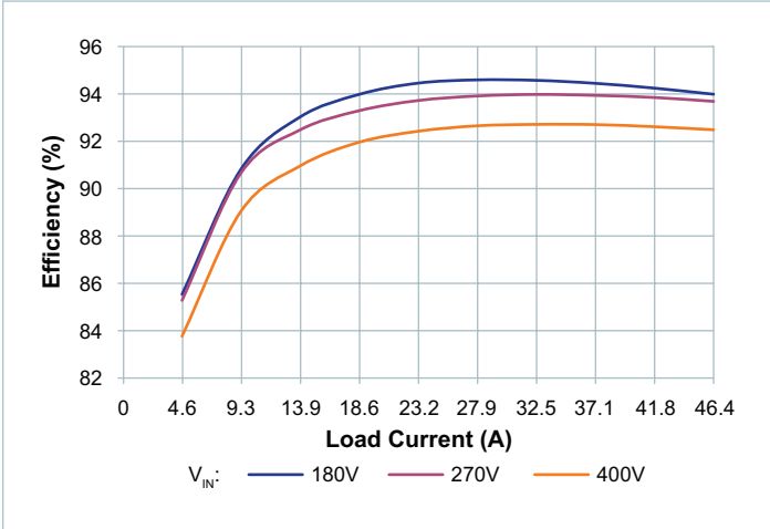
Figure 8 — Efficiency vs. load at T_{CASE} = -40^{\circ}C , nominal trim
