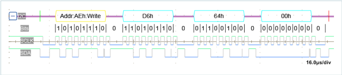
Figure 27 — TON_DELAY COMMAND (60h)_WRITE WORD PROTOCOL
