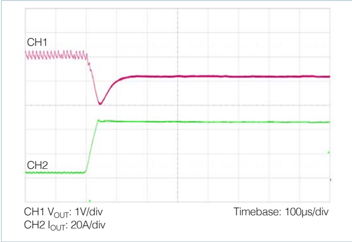
Figure 21 — 10 – 100% load transient response, V_{IN} = 270V , nominal trim, C_{OUT\_EXT} = 0\mu F
