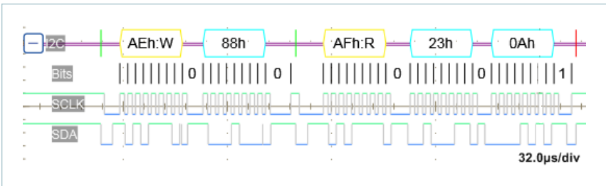
Figure 28 — MFR_VIN_MIN COMMAND (A0h)_READ WORD PROTOCOL
