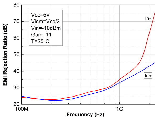
Figure 43. EMIRR on In+, In- and Out pins
