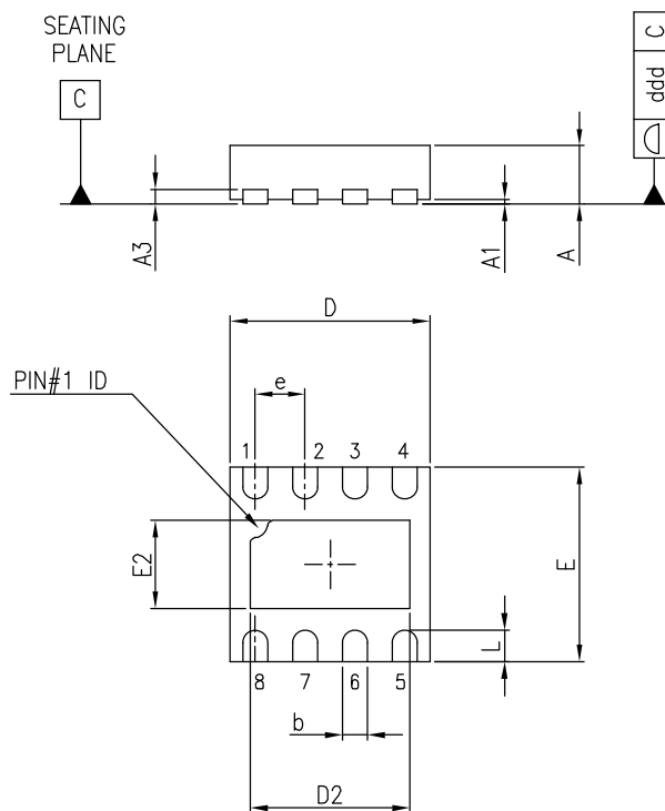
Figure 50. DFN8 2x2 package outline
