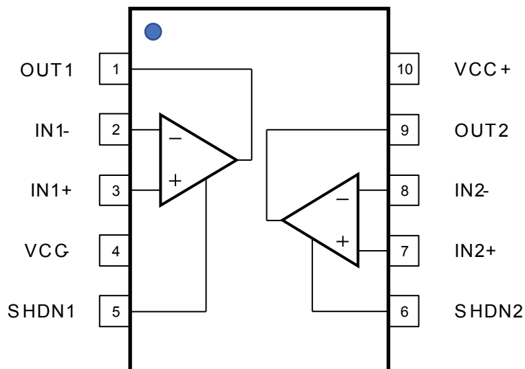
Figure 3. Pin connections (top view)
