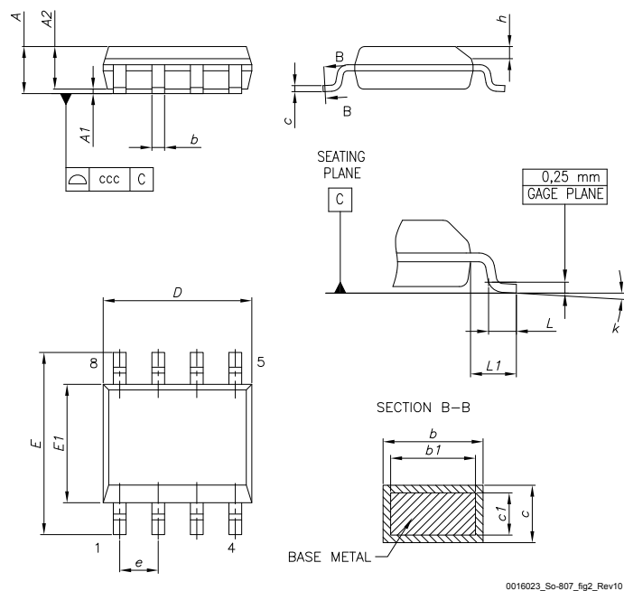
Figure 53. SO-8 package outline
