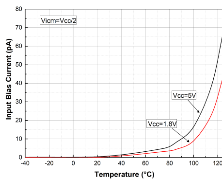
Figure 14. Input bias current vs. temp. at V_{ICM} = V_{CC} / 2
