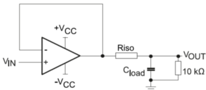
Figure 44. Test configuration for R_{ISO}
