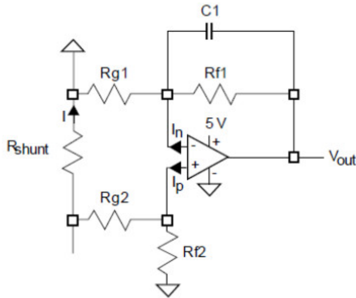
Figure 47. Low-side current sensing schematic
