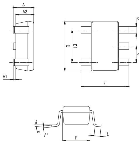
Figure 49. SOT23-5 package outline
