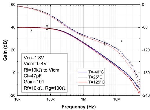
Figure 26. Closed loop bode diagram at V_{CC} = 1.8\text{ V}
