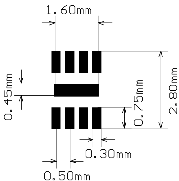
Figure 51. DFN8 2x2 recommended footprint
