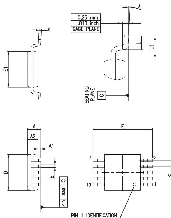
Figure 54. MiniSO10 package outline
