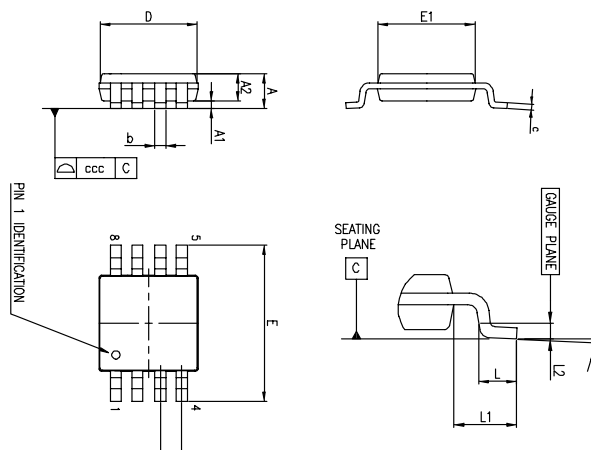
Figure 52. MiniSO8 package outline
