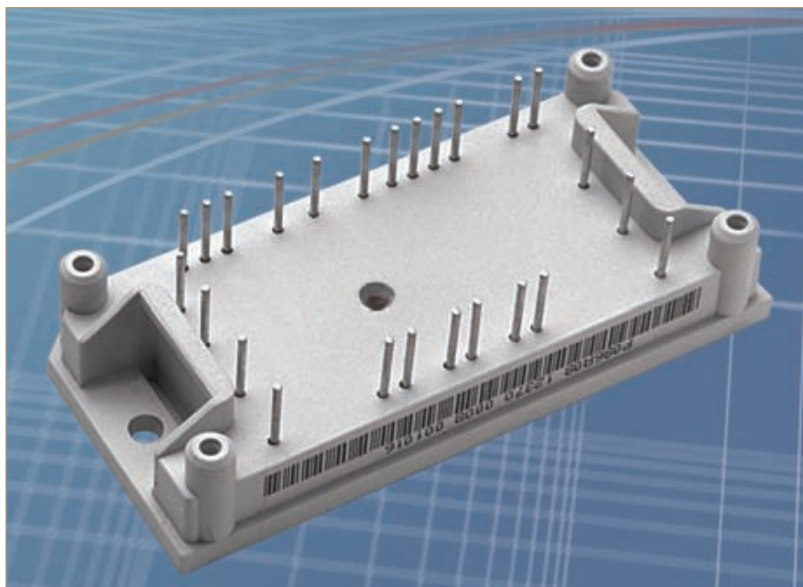
Figure 3: Half-bridge module with 1200V and 100A rating optimised for fast switching applications
