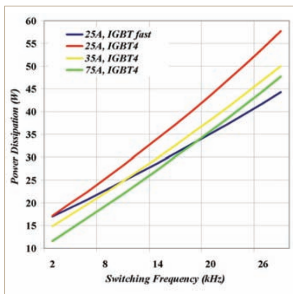
Figure 1: Total power dissipation of different IGBTs as a function of switching frequency (10kW DC link power, 50Hz output motor frequency)
