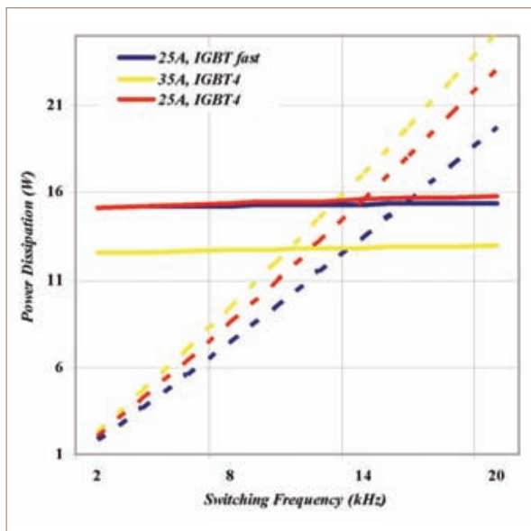
Figure 2: Static (solid) and dynamic (dotted) losses as a function of switching frequency (10kW DC link power, 50Hz output motor frequency)
